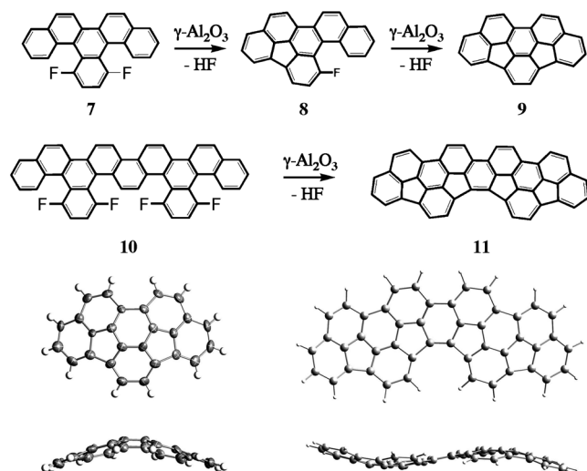
Figure 3. Synthesis of buckybowls by the CRC approach. Top: Buckybowl synthesis by two- and fourfold cove-region closure. Bottom: ORTEP of compound 9 (top and side view) and DFT optimized structure of 11 (top and side view), demonstrating the geodesic shapes. Compounds 9 and 11 were obtained in quantitative yield.
